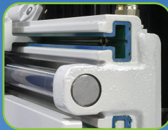
Fully enclosed wrap around UHMW bearings
